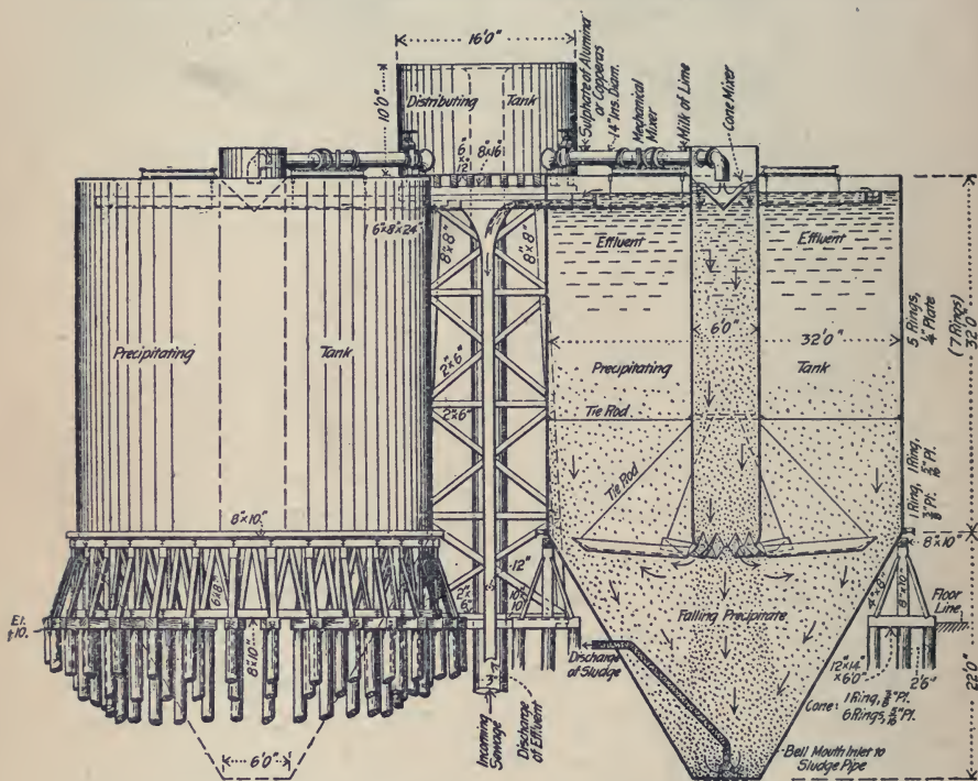
FIG. 37.—ELEVATION AND SECTION OF RECEIVING AND PRECIPITATING TANKS.
